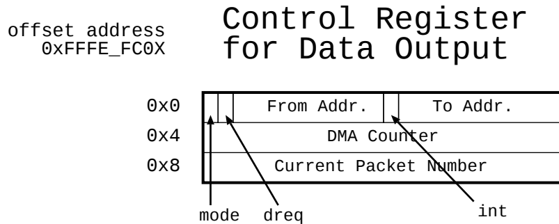
図 23.14: Data Out Control Register
