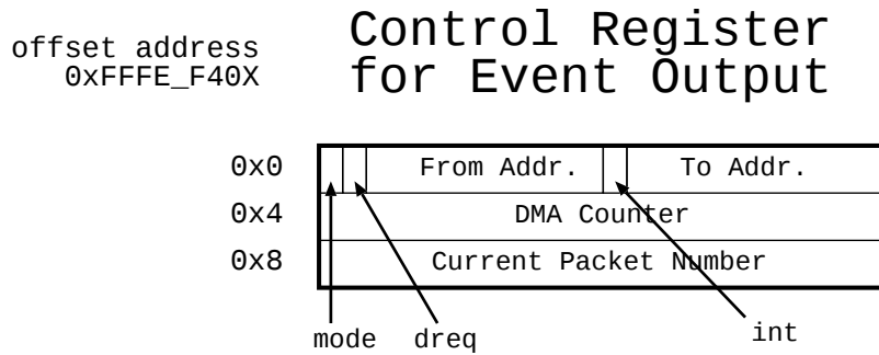
図 23.10: Event Out Control Register
