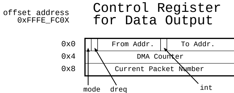
図 26.14: Data Out Control Register
