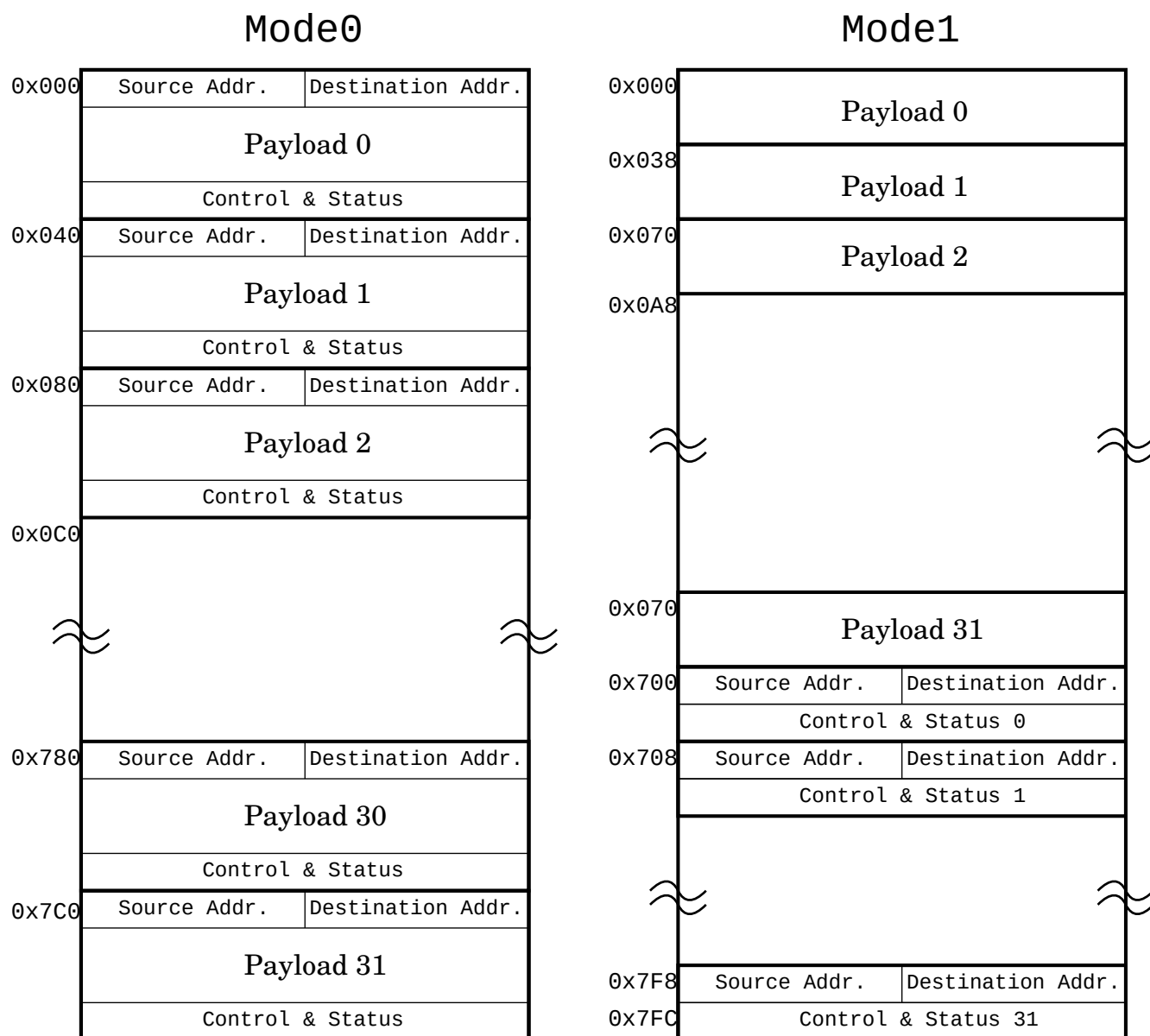
☒ 26.15: DPM for Data Input
