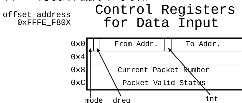
☒ 26.16: Data In Control Register
