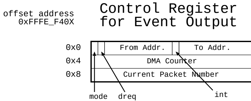
図 26.10: Event Out Control Register
